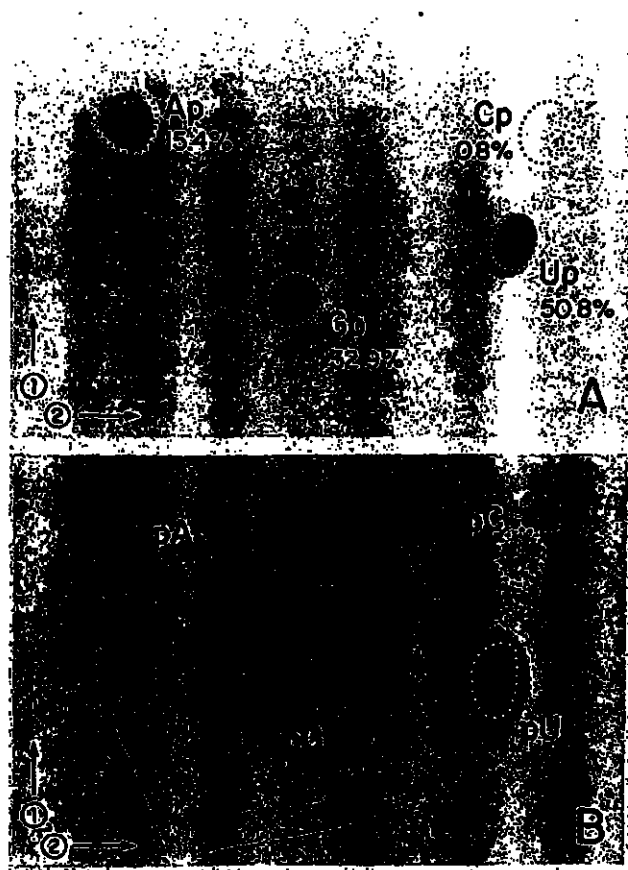
Fig. 2. Nearest neighbour and nucleotide analyses of internally incorporated [ \alpha - ^{32} P]UTP. (A and B) pNB2 RNA labeled with [ \alpha - ^{32} P]UTP in the presence of TL extract was digested with RNase H and the oligomer S165. The 5' fragment was gel-isolated, digested with RNase T2 (A) or nuclease P1 (B) and the resulting 3' monophosphates (A) or 5' monophosphates (B) separated by 2-D TLC. The relative amounts of label in each of the 3' monophosphate spots are indicated.
