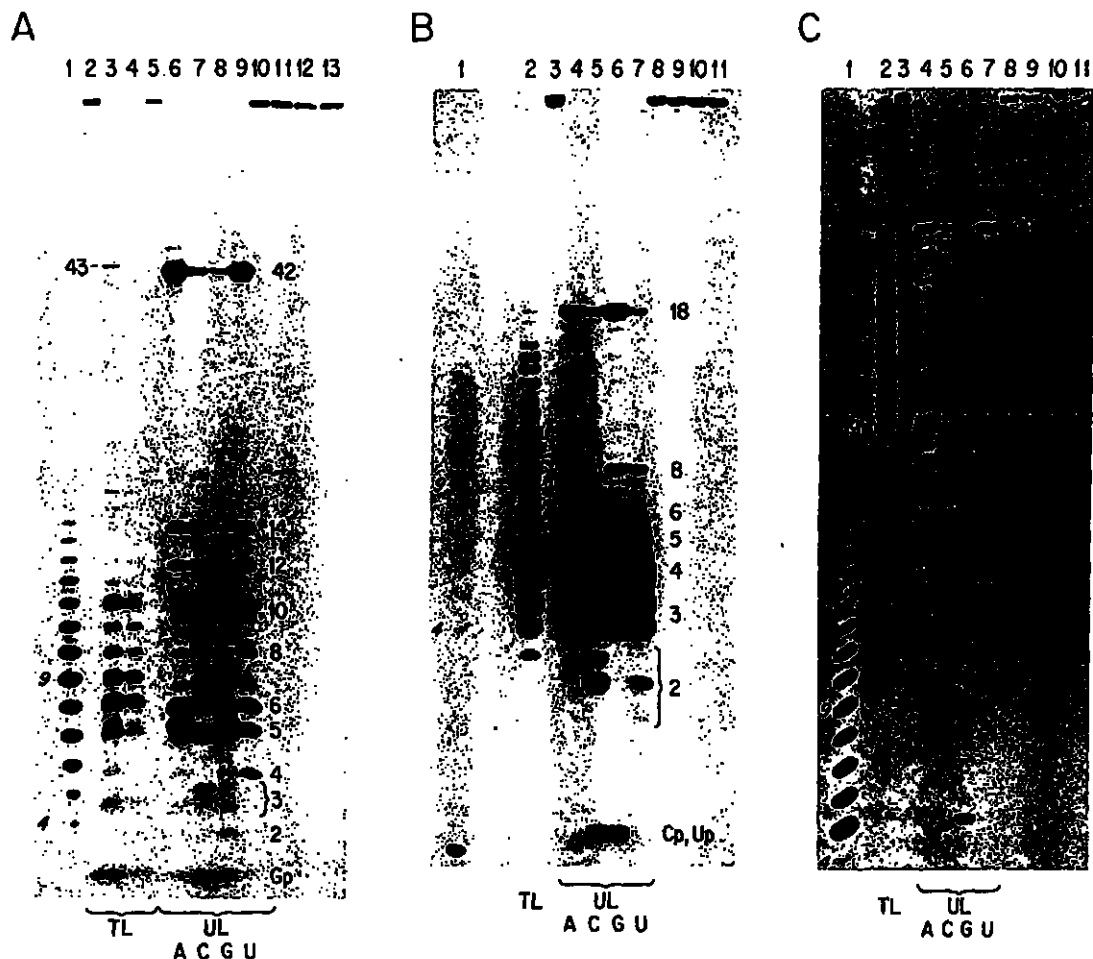
Fig. 3. Fingerprinting analyses of pNB2 RNA containing internal U-incorporations. (A,B,C) pNB2 RNA was either uniformly labeled (UL) with [ \alpha - ^{32} P]ATP, [ \alpha - ^{32} P]CTP, [ \alpha - ^{32} P]GTP or [ \alpha - ^{32} P]UTP to obtain control substrates, or labeled by incubation with TL extract in the presence of [ \alpha - ^{32} P]UTP. The 5' portions were recovered after cleavage with RNase H in conjunction with the oligomer S1025, and used for nuclease digestion and subsequent PAGE analysis. Sizes of predicted RNA oligomers appear on the right, and the positions of oligo(dT) 4mers and 9mers are indicated italicized on the left of each panel. (A) Digestion with RNase T1. Two different TL extracts were used for this experiment and the data obtained were qualitatively equivalent (lanes 3 and 4). Lane 1, oligo (dT) 4-22 ladder; lanes 2 and 5, TL-incubated RNA, 0 min time points of digests shown in lanes 3 and 4; lanes 6-9, UL RNA, labeled as indicated with A, C, G or U, digested with RNase T1; lanes 10-13, 0 min time points of control digests shown in lanes 6-9. (B) RNase A digestion. Lane 1, (dT) 4-22 ; lane 2, TL-incubated RNA digested with RNase A; lane 3, 0 min time point of TL-incubated RNA shown in lane 2; lanes 4-7, UL controls, labeled as indicated, digested with RNase A; lanes 8-11, 0 min time points of digests shown in lanes 4-7. (C) Digestion with RNase CL3. Lane 1, (dT) 4-22 ; lane 2, TL-incubated RNA digested with RNase CL3; lane 3, 0 min time point of TL-incubated RNA shown in lane 2; lanes 4-7, UL RNA, labeled as indicated, digested with RNase CL3; lanes 8-11, 0 min time points of digests shown in lanes 4-7.
