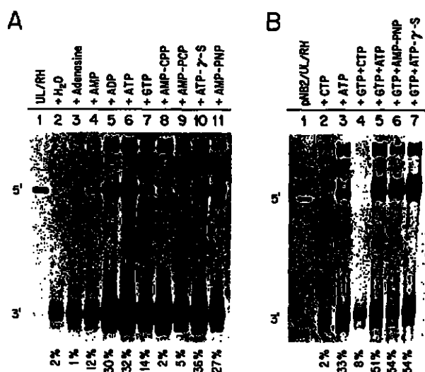
Fig. 5. Nucleotide requirements of internal U-incorporation activity. (A and B) pNB2 RNA uniformly labeled (lane 1) or labeled by incubation with TL (lanes 2–11) was analyzed by the RNase H assay in conjunction with oligomer S165. Incubation with TL was performed under standard conditions, except that only the indicated cold triphosphates were present at 1 mM each. The relative percentages of label incorporation (5' internal versus 3' addition) as well as the positions of the 5' and 3' fragments are indicated.
