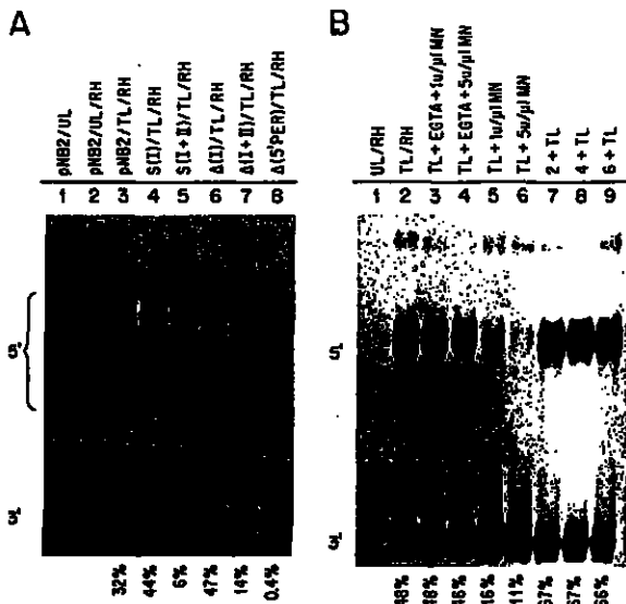
Fig. 6. Removal/modification of CYb mRNA anchor sequences, and micrococcal nuclease digestion. (A) pNB2 RNA or RNA from each of the five mutants was labeled with [ \alpha - ^{32} P]UTP by incubation with TL and subsequently analyzed by the RNase H assay using oligomer S165 (lanes 3–8). The relative percentages of label incorporation (5' internal versus 3' addition) are indicated. Uniformly labeled pNB2 RNA was used as a control (lanes 1 and 2). (B) TL extract was incubated with active micrococcal nuclease (MN) (lanes 5 and 6), or EGTA-inactivated MN (lanes 3 and 4). After EGTA-inactivation of the nuclease in all samples, \Delta (I) RNA was added and labeled with [ \alpha - ^{32} P]UTP under standard incubation conditions. \Delta (I) RNA labeled by incubation with untreated TL extract served as a positive control (lane 2). Samples pretreated as those shown in lanes 2, 4 or 6 were incubated with an equal amount of fresh TL extract (lanes 7–9). All reactions were subsequently analyzed by the RNase H assay in conjunction with oligomer S165. The micrococcal nuclease concentrations are indicated, as well as the relative percentages of label incorporation (5' internal versus 3' addition). RNase H-digested uniformly labeled \Delta (I) RNA was run as a size marker (lane 1).
