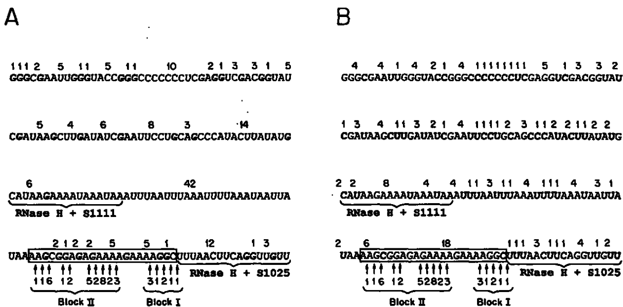
Fig. 4. Predicted fragment sizes of pNB2 RNA digested with RNase T1 or RNase A. (A and B) The sequence of the pNB2 RNA 5' portion used for the fingerprinting analyses in Figure 3 is indicated. The predicted digestion fragment sizes appear above the sequence, flanked by emboldened G nucleotides (A), or emboldened C and U nucleotides (B), 3' of which RNase T1 or RNase A, respectively, are expected to cleave. The localizations of the DNA oligonucleotides S1111 and S1025 used for RNase H cleavage, as well as the sites and numbers of U additions in mature edited CYb mRNA are shown. Block I and II within the boxed pre-edited region refer to the two editing blocks.
