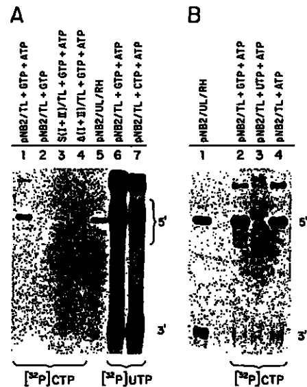
Fig. 7. Internal C-incorporation into pNB2 RNA. (A) pNB2 RNA was labeled using TL and [ \alpha - ^{32} P]CTP (lanes 1 and 2) or [ \alpha - ^{32} P]UTP (lanes 6 and 7). S(I+II) RNA (lane 3) and \Delta (I+II) RNA (lane 4) were labeled using TL and [ \alpha - ^{32} P]CTP. Uniformly labeled pNB2 RNA served as a control (lane 5). All reactions were analyzed by the RNase H assay in conjunction with oligomer S165. The various cold triphosphates (1 mM each) added to the reactions are indicated. (B) pNB2 RNA uniformly labeled (lane 1) or labeled by incubation with TL and [ \alpha - ^{32} P]CTP (lanes 2–4) was analyzed by the RNase H assay in conjunction with oligomer S165. The various cold triphosphates (1 mM each) added to the reactions are indicated.
