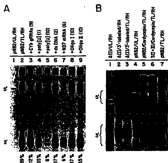
Fig. 8. Specific inhibition of internal U-incorporation by RNA, and lack of U-internalization from the 3' end of pNB2 RNA. (A) pNB2 RNA was labeled with [\alpha\text{-}^{32}\text{P}]\text{UTP} by incubation with TL in the presence of cold synthetic CYb gRNAs I and II (lane 3), poly(U) (lanes 4 and 5), an 87 bp PCR fragment (lane 6), synthetic ND7 mRNA (lane 7), two different oligodeoxynucleotides (lanes 8 and 9) or without addition of heterologous RNA (lane 2). The numbers in parentheses indicate the number of pmol nucleic acids added. Five pmol of pNB2 substrate RNA was present in each reaction. Uniformly labeled pNB2 RNA served as a control (lane 1). All reactions were analyzed by the RNase H assay using oligomer S165. The relative percentages of label incorporation (5' internal versus 3' addition) are indicated. (B) pNB2 RNA or S(I+II) RNA containing cordycepin (3' deoxyadenosine) at the 3' ends (lanes 5 and 6) were labeled with [\alpha\text{-}^{32}\text{P}]\text{UTP} by incubation with TL and subsequently analyzed by the RNase H assay in conjunction with oligomer S165. Gel-isolated, [\alpha\text{-}^{32}\text{P}]\text{UTP} 3' end-labeled \Delta(I) RNA was either directly digested with RNase H (lane 2), or first incubated with TL in the absence of [\alpha\text{-}^{32}\text{P}]\text{UTP} (lane 3). pNB2 RNA without cordycepin served as a control for the activity of the TL extract (lane 7). RNase H-digested uniformly labeled \Delta(I) RNA (lane 1) and pNB2 RNA (lane 4) were run as size markers.
