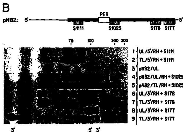
Fig. 1. U-incorporation into synthetic pNB2 and ND7 RNAs.
